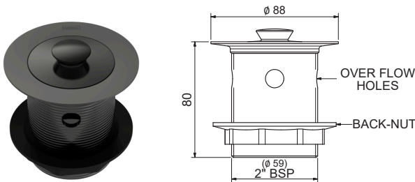
ANELLO 50MM SINK/BATH WASTE – OVERFLOW AP&W50O + [Finish Code]
