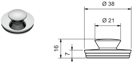
32MM ANELLO STOPPER AS32 + [Finish Code]
