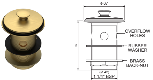
MERINO 32MM BASIN WASTE – OVERFLOW MP&W32O + [Finish Code]
