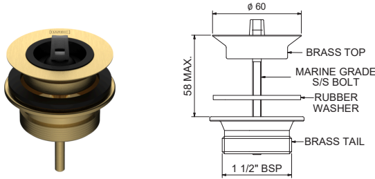
2 PART TAPERED BASIN WASTE 32MM TOP, 40MM BSP BASE PWT32-40 + [Finish Code]
