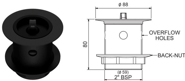
50MM SINK/BATH WASTE WITH RUBBER PLUG, 80MM TAIL – OVERFLOW PW5080O + [Finish Code]
