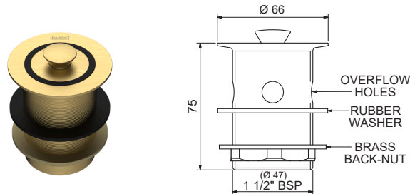
BOWEN 40MM BASIN/BATH WASTE – OVERFLOW BP&W40O + [Finish Code]
