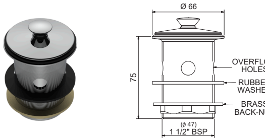
MERINO 40MM BASIN/BATH WASTE – OVERFLOW MP&W40O + [Finish Code]
