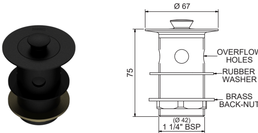
ANELLO 32MM BASIN WASTE – OVERFLOW AP&W32O + [Finish Code]
