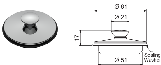
50MM MERINO STOPPER MS50 + [Finish Code]
