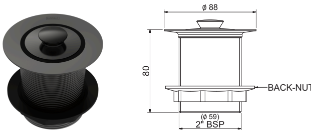
BOWEN 50MM SINK/BATH WASTE BP&W50 + [Finish Code]
