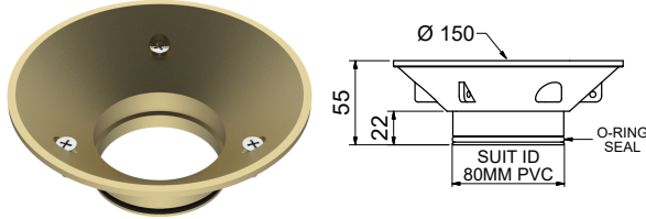
VINYL FLOOR WASTE BASE - 80MM VFWBP80BR
