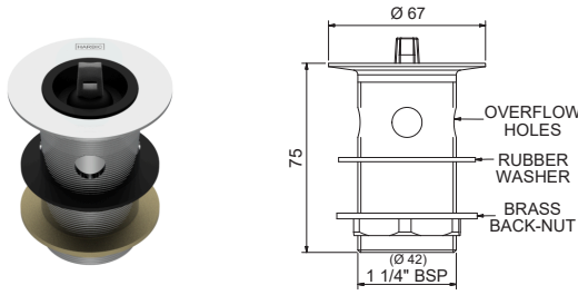
32MM BASIN WASTE WITH RUBBER PLUG, 80MM TAIL – OVERFLOW PW3280O + [Finish Code]
