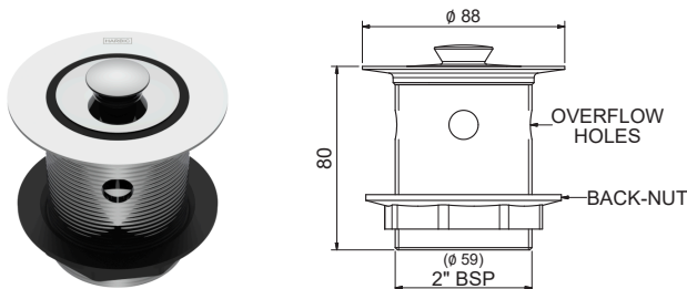
BOWEN 50MM SINK/BATH WASTE – OVERFLOW BP&W50O + [Finish Code]
