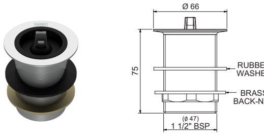
40MM BASIN/BATH WASTE WITH RUBBER PLUG, 80MM TAIL PW4080 + [Finish Code]
