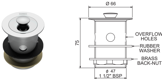
ANELLO 40MM BASIN/BATH WASTE – OVERFLOW AP&W40O + [Finish Code]
