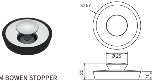
50MM BOWEN STOPPER BS50 + [Finish Code]
