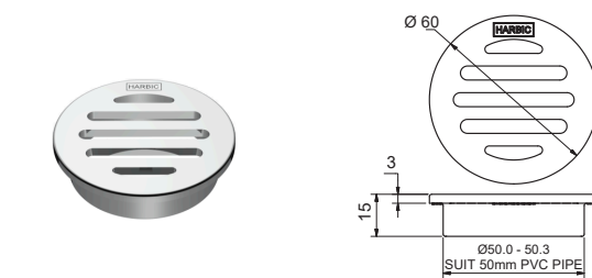
PLAIN PATTERN FLOOR WASTE ROUND TOP SUIT 50MM PVC FWP50CP
