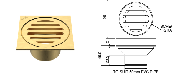
CUP PATTERN FLOOR WASTE SQUARE TOP SUITS 50MM PVC FWC50PT + [Finish Code]
