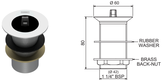
32MM TAPERED BASIN WASTE WITH RUBBER PLUG, 80MM TAIL PWT3280 + [Finish Code]
