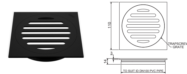
FLOOR WASTE SQUARE TOP SUITS 100MM PVC TSG100PT + [Finish Code]
