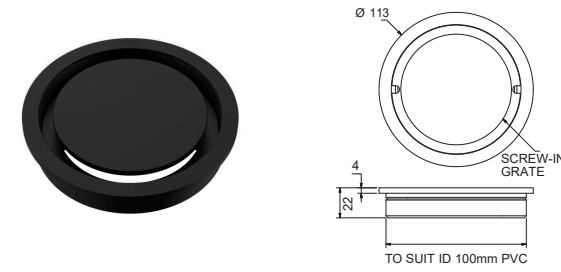
HALO FLOOR WASTE ROUND TOP SUITS 100MM PVC HALTSG100P + [Finish Code]
