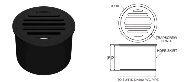
LEAK CONTROL FLOOR WASTE ROUND TOP SUITS 100MM PVC FWLCF100 + [Finish Code]
