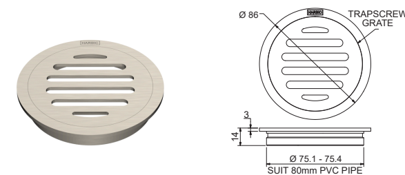
FLOOR WASTE ROUND TOP SUITS 80MM PVC TSG80P + [Finish Code]
