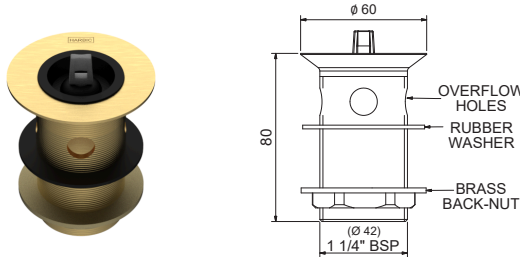
32MM TAPERED BASIN WASTE WITH RUBBER PLUG, 80MM TAIL – OVERFLOW PWT3280O + [Finish Code]
