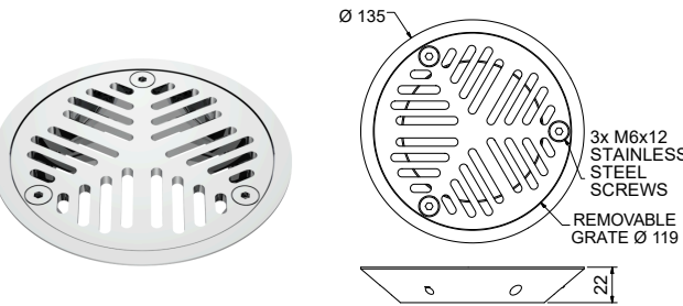
CLAMP RING & GRATE FOR 100MM BASE VFWRG100CP
