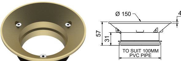
VINYL FLOOR WASTE BASE - 100MM VFWBP100BR
