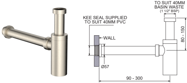
BOTTLE TRAP - 40MM BTR40 + [Finish Code]
