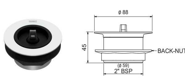
50MM SINK/BATH WASTE WITH RUBBER PLUG, 45MM TAIL PW5045 + [Finish Code]
