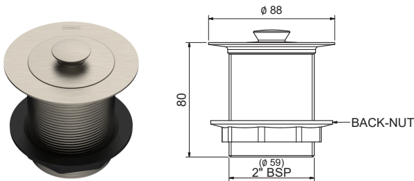
ANELLO 50MM SINK/BATH WASTE AP&W50 + [Finish Code]
