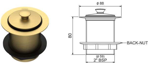
MERINO 50MM SINK/BATH WASTE MP&W50 + [Finish Code]
