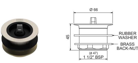
40MM BASIN/BATH WASTE WITH RUBBER PLUG, 45MM TAIL PW4045 + [Finish Code]
