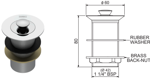
ANELLO 32MM TAPERED BASIN WASTE AP&WT32 + [Finish Code]
