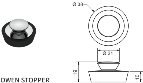
32MM BOWEN STOPPER BS32 + [Finish Code]
