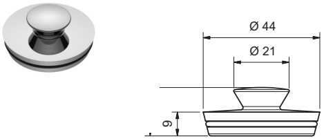
40MM ANELLO STOPPER AS40 + [Finish Code]
