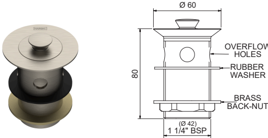
ANELLO 32MM TAPERED BASIN WASTE – OVERFLOW AP&WT32O + [Finish Code]
