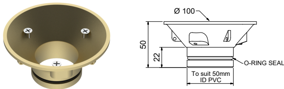
VINYL FLOOR WASTE BASE - 50MM VFWBP50BR
