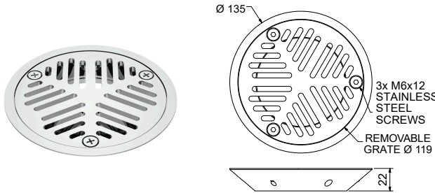
CLAMP RING & GRATE FOR 80MM BASE VFWRG80CP
