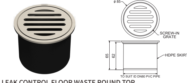
LEAK CONTROL FLOOR WASTE ROUND TOP SUITS 80MM PVC FWLCF80 + [Finish Code]
