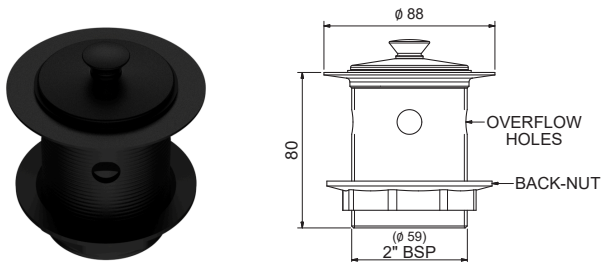
MERINO 50MM SINK/BATH WASTE – OVERFLOW MP&W50O + [Finish Code]
