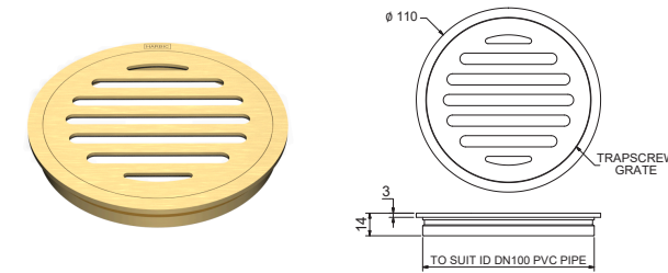
FLOOR WASTE ROUND TOP SUITS 100MM PVC TSG100P + [Finish Code]
