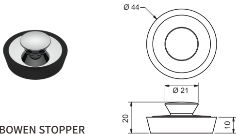
40MM BOWEN STOPPER BS40 + [Finish Code]
