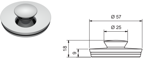
50MM ANELLO STOPPER AS50 + [Finish Code]
