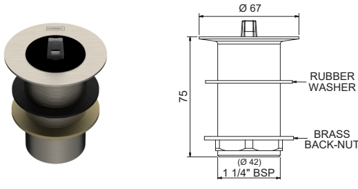
32MM BASIN WASTE WITH RUBBER PLUG, 80MM TAIL PW3280 + [Finish Code]
