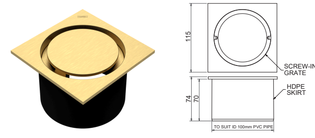
HALO LEAK CONTROL FLOOR WASTE SQUARE TOP SUITS 100MM PVC HALFWLCF100T + [Finish Code]
