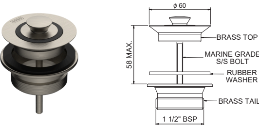
BOWEN 2 PART TAPERED BASIN WASTE 32MM TOP, 40MM BSP BASE BP&WT32-40 + [Finish Code]
