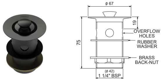
BOWEN 32MM BASIN WASTE – OVERFLOW BP&W32O + [Finish Code]
