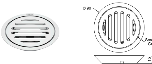
CLAMP RING & GRATE FOR 50MM BASE VFWRG50CP
