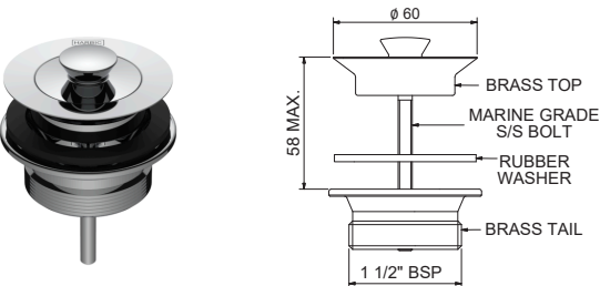
ANELLO 2 PART TAPERED BASIN WASTE 32MM TOP, 40MM BSP BASE AP&WT32-40 + [Finish Code]
