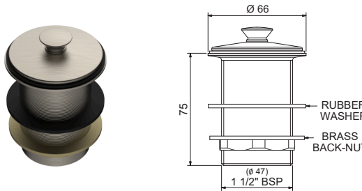
MERINO 40MM BASIN/BATH WASTE MP&W40 + [Finish Code]
