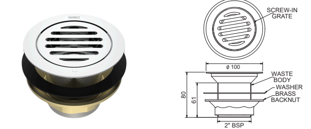
SHOWER WASTE ROUND TOP 50 X 80 PRESSED STEEL, ACRYLIC, & FIBREGLOSS SHOWERS SW5080CP
