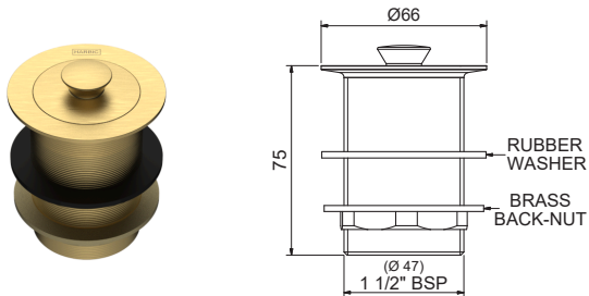
ANELLO 40MM BASIN/BATH WASTE AP&W40 + [Finish Code]
