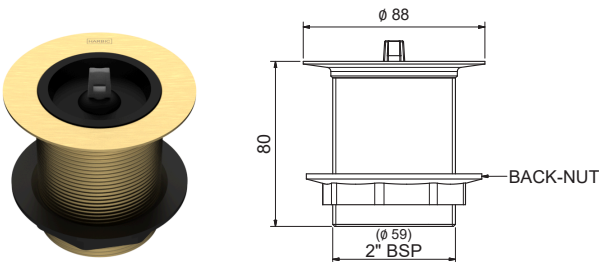
50MM SINK/BATH WASTE WITH RUBBER PLUG, 80MM TAIL PW5080 + [Finish Code]
