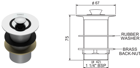
BOWEN 32MM BASIN WASTE BP&W32 + [Finish Code]
