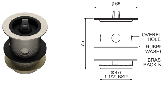
40MM BASIN/BATH WASTE WITH RUBBER PLUG, 80MM TAIL – OVERFLOW PW4080O + [Finish Code]
