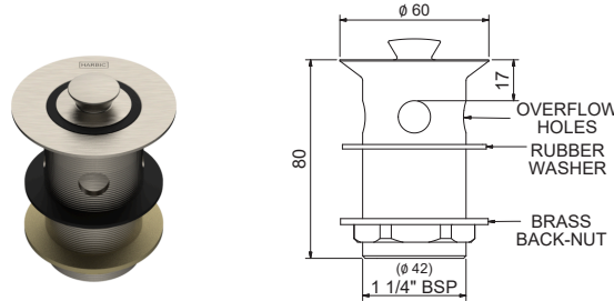
BOWEN 32MM TAPERED BASIN WASTE – OVERFLOW BP&WT32O + [Finish Code]
