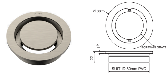
HALO FLOOR WASTE ROUND TOP SUITS 80MM PVC HALTSG80P + [Finish Code]
