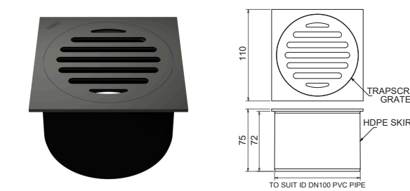
LEAK CONTROL FLOOR WASTE SQUARE TOP SUITS 100MM PVC FWLCF100T + [Finish Code]
