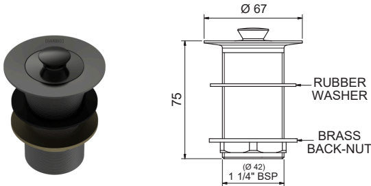
ANELLO 32MM BASIN WASTE AP&W32 + [Finish Code]
