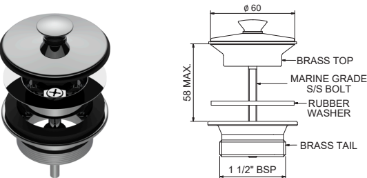
MERINO 2 PART TAPERED BASIN WASTE 32MM TOP, 40MM BSP BASE MP&WT32-40 + [Finish Code]
