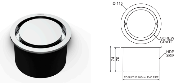
HALO LEAK CONTROL FLOOR WASTE ROUND TOP SUITS 100MM PVC HALFWLCF100 + [Finish Code]
