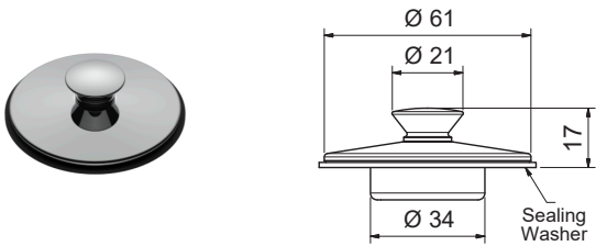
40MM MERINO STOPPER (SUITS 32MM & 40MM WASTES) MS40 + [Finish Code]
