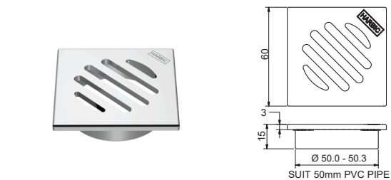
PLAIN PATTERN FLOOR WASTE SQUARE TOP SUIT 50MM PVC FWP50TCP
