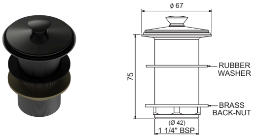
MERINO 32MM BASIN WASTE MP&W32 + [Finish Code]
