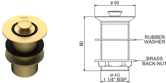
BOWEN 32MM TAPERED BASIN WASTE BP&WT32 + [Finish Code]
