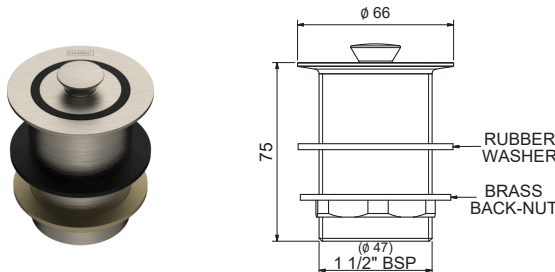
BOWEN 40MM BASIN/BATH WASTE BP&W40 + [Finish Code]
