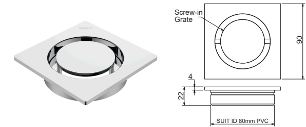
HALO FLOOR WASTE SQUARE TOP SUITS 80MM PVC HALTSG80PT + [Finish Code]
