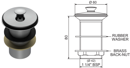
MERINO 32MM TAPERED BASIN WASTE MP&WT32 + [Finish Code]
