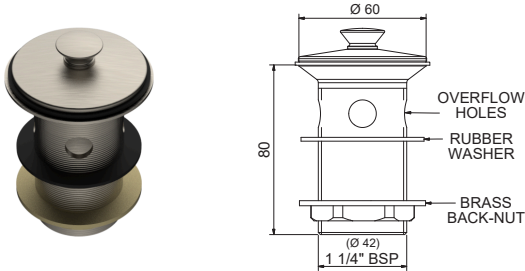
MERINO 32MM TAPERED BASIN WASTE – OVERFLOW MP&WT32O + [Finish Code]
