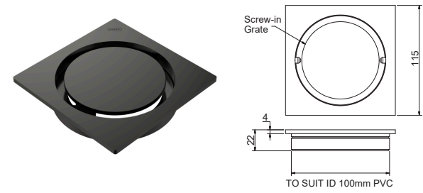
HALO FLOOR WASTE SQUARE TOP SUITS 100MM PVC HALTSG100PT + [Finish Code]
