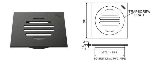
FLOOR WASTE SQUARE TOP SUITS 80MM PVC TSG80PT + [Finish Code]
